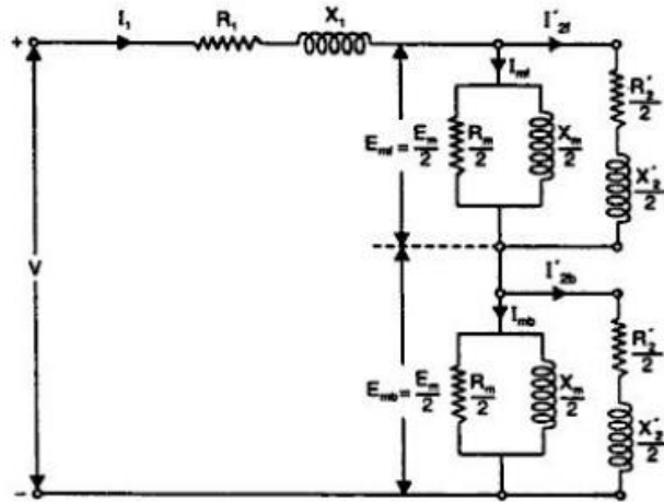
Fig:5.6 (b) Equivalent Circuit of Single Phase Induction Motor at Standstill on the basis of Two Revolving Field Theory
