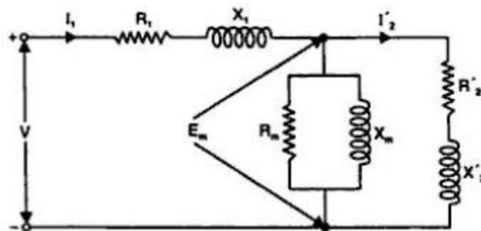
Fig:5.6 (a) Equivalent Circuit of a Single Phase Induction Motor
