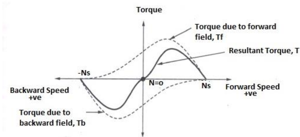
Fig: 5.5.1(g) Torque-Speed characteristics
